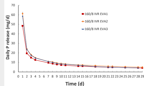
Fig. 2. Dissolution of P from segmented IVRs (160/80) prepared from 28% vinyl acetate content EVA from three different suppliers.
